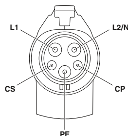
Type 1 vehicle charging connector pin assignment
