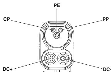
Vehicle charging connector pin assignment
