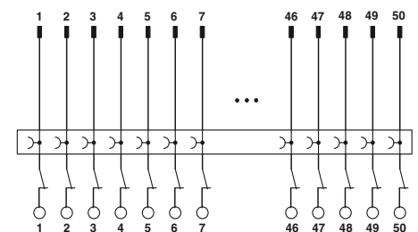
Connection scheme FLKM 50/KDS3-MT/PPA/AN/PLC
