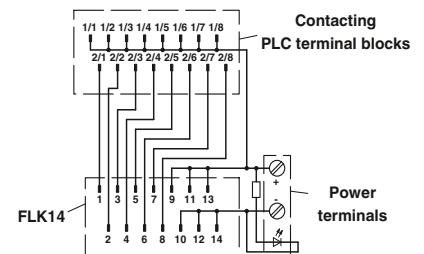
Connection scheme PLC-V8/FLK14/OUT/M
