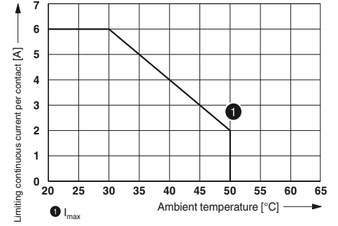
Contact derating
