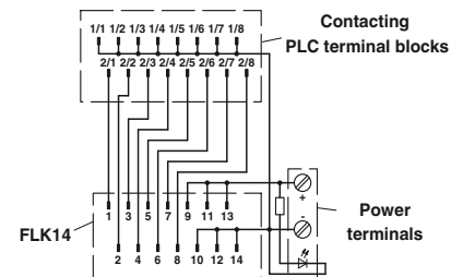
Connection scheme PLC-V8/FLK14/IN/M
