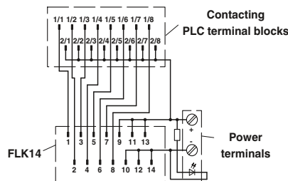
Connection scheme PLC-V8/FLK14/IN
