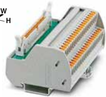
Passive termination board For Modicon® TSX Quantum™ with Push-in connection
