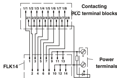
Connection scheme PLC-V8/FLK14/OUT
