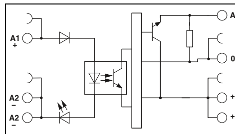
Solid-state relay module, DC output, transmission frequency of 100 kHz
