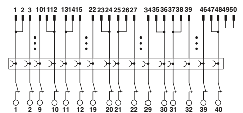
Connection scheme FLKM 50/KDS3-MT/PPA/S7-300
