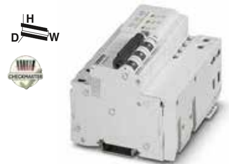
4-conductor system; L1, L2, L3, PEN with integrated backup fuse
