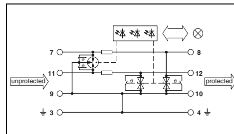
2-conductor with common reference potential, connection 9/10 grounded directly, e.g., for binary signals
