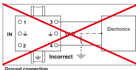
Ground connection
