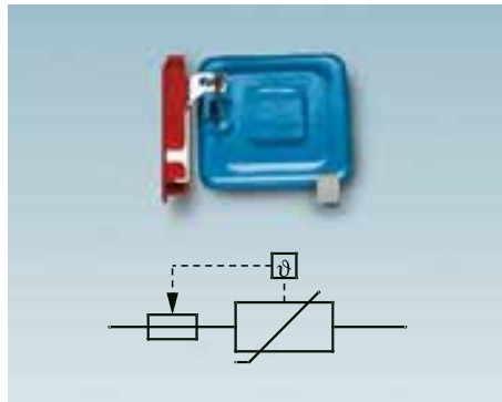
Block varistor with thermal disconnect device
