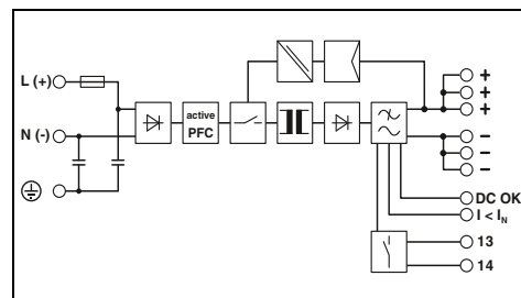
Power supply, with protective coating, 1 AC, 24 V DC, 5 A
