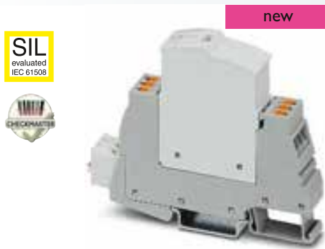
3-conductor system, L, N, PE or DC+, DC-, PE, 60 V nominal voltage
