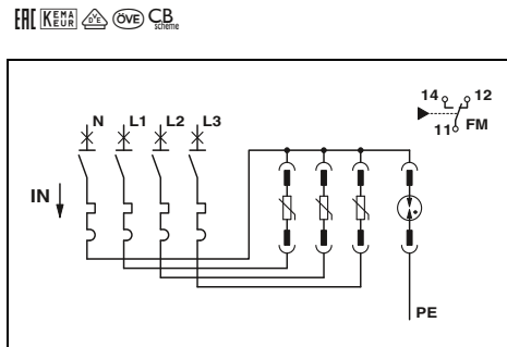
5-conductor system; L1, L2, L3, N, PE with integrated backup fuse
