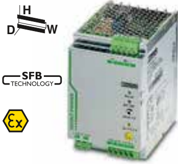
DC/DC converter, with protective coating, 24 V DC/24 V DC, 20 A
