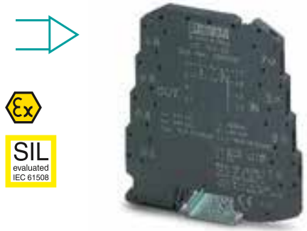
Double wire (loop), floating, e.g., for 4 ... 20 mA current loops
