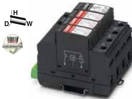
5-conductor system; L1, L2, L3, N, PE, supply line supply from below
