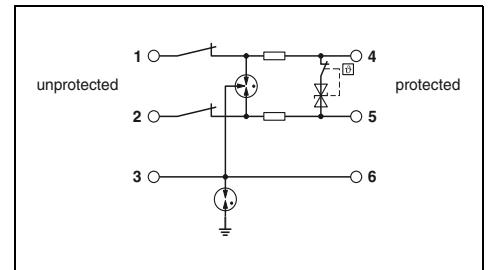
Double wire (loop), floating, 3/6 connection grounded via gas-filled surge arrester, with knife disconnection, e.g., for 4 ... 20mA current loop
