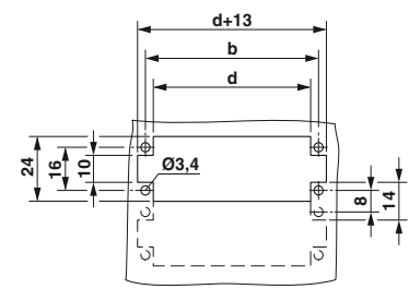
Panel cutout
