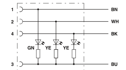
Contact assignment of M12 female connectors with LED
