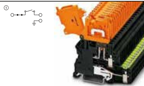
20 A, lever-type disconnect terminal block, same shape, with PE foot
