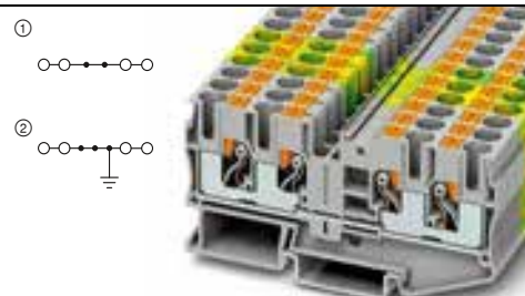
52 A, feed-through terminal block, 4 connections
