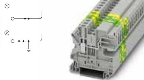
32 A, feed-through terminal block, horizontal plug-in connection
