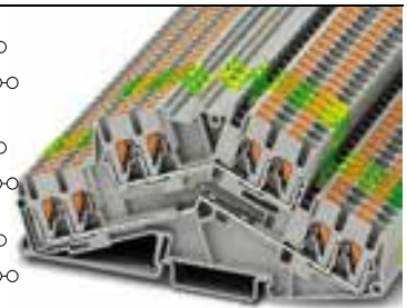
24 A, double-level terminal block, 4 connections per level
