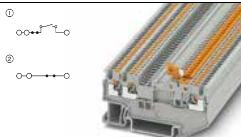
10 A, knife disconnect terminal block, 3 connections
