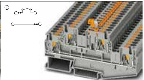
32 A, double-level knife disconnect terminal block, one disconnect zone
