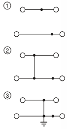
26 A, double-level terminal block, 4 connections
