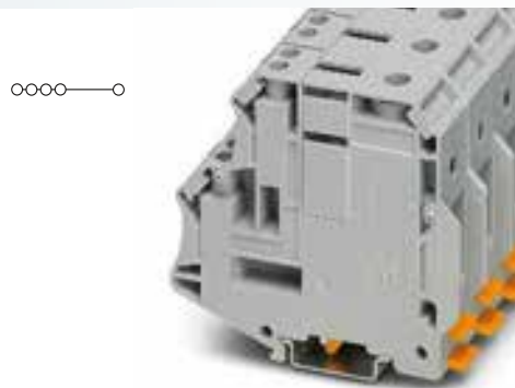
192 A, potential collective terminal, 4 inputs 10 mm 2
