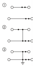
16 A, double-level terminal block
