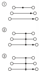
15 A, multi-level terminal block, 6 connections
