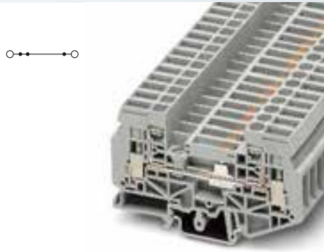
6 (10) mm 2 , 57 A, slide-type terminal block
