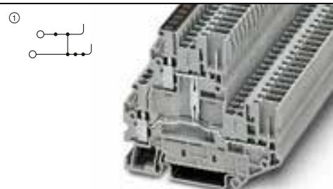
24 A, double-level terminal block with equipotential bonder
