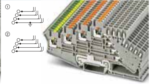
10 A, four-level terminal block with PE foot
