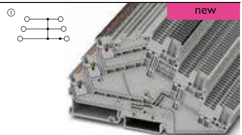
15 A, three-level terminal block with potential distribution
