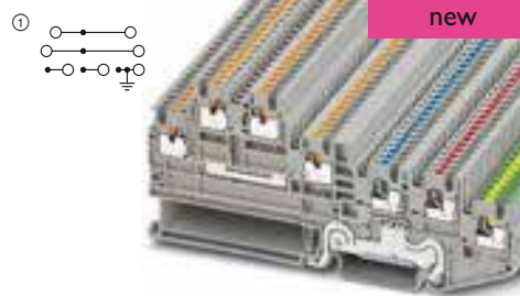
13.5 A, five-conductor actuator terminal block, with PE foot
