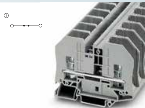
125 A, feed-through terminal block, open
