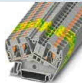
38 A, feed-through terminal block, 3 connections
