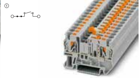
20 A, knife disconnect terminal block
