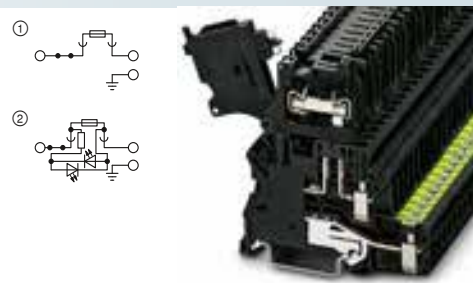
6.3 A, lever-type fuse terminal block for 5 x 20 mm cartridge fuses, with PE foot
