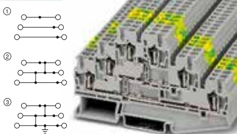
28 A, three-level terminal block
