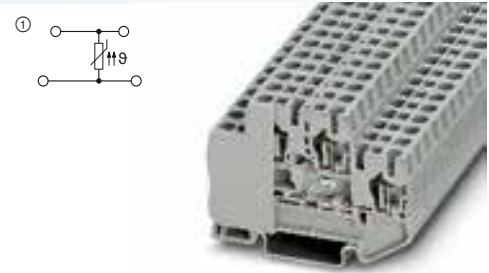
26 A, double-level terminal block with temperature sensor
