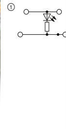
24 A, double-level terminal block with LED display
