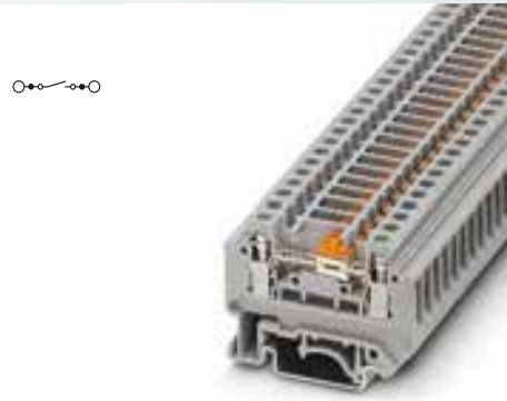
4 (4) mm 2 , 26 A, disconnect terminal block
