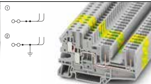
32 A, feed-through terminal block, 4 connections
