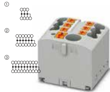
57 A, adhesive mounting
