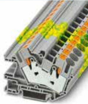
76 A, feed-through terminal block
