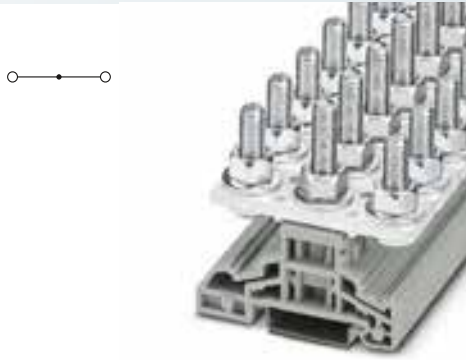
50 (50) mm 2 , 150 A, M8 bolt terminal block
