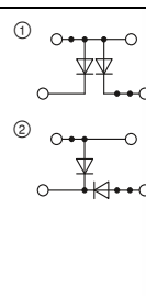
28 A, double-level terminal block with two 1N 4007 diodes (1300 V/0.5 A)
