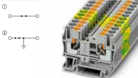
52 A, feed-through terminal block
