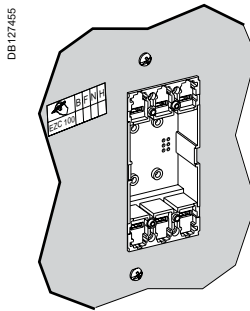
Front connection.
