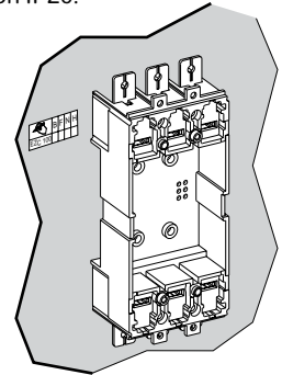
Fixation on rear plate.
