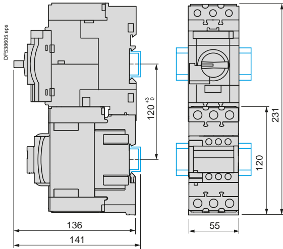
Vertical mounting (1)
