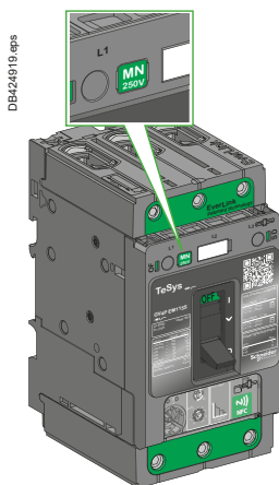
DB424915.eps Visible presence of MN undervoltage release in circuit breaker cavity, visible rated voltage through the window.
