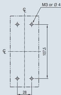
Panel drilling
