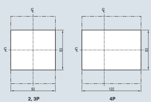
Front panel cutting
